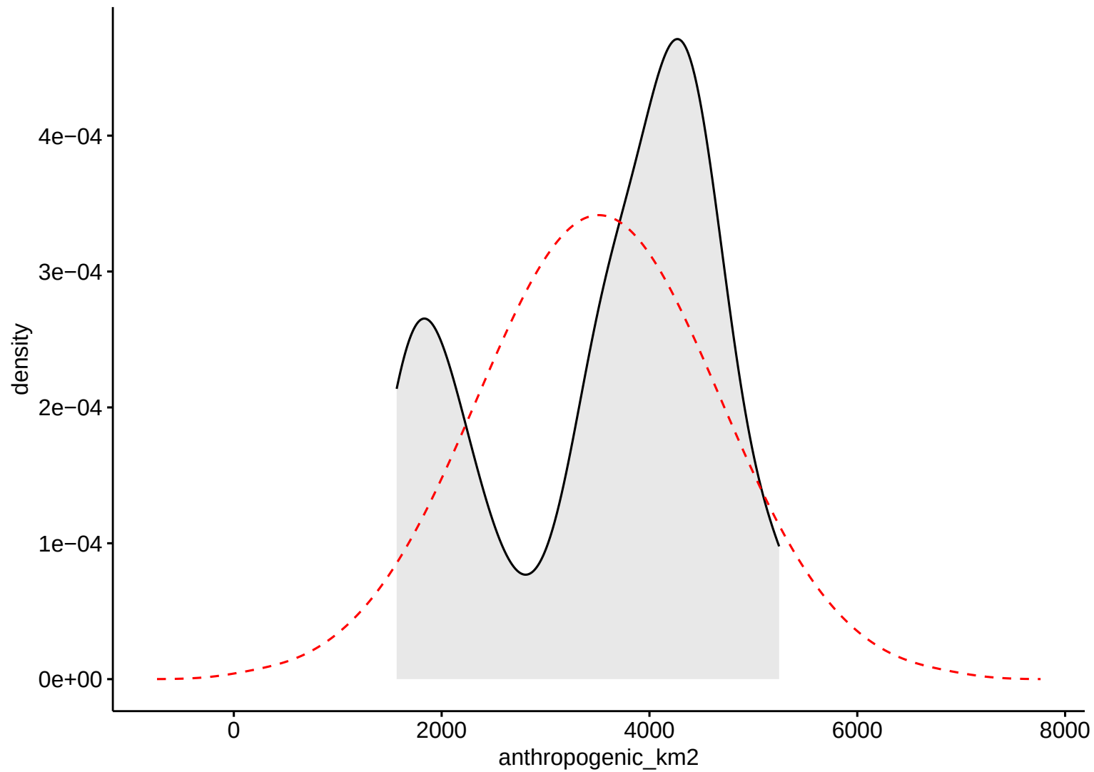
Anthropic Area
